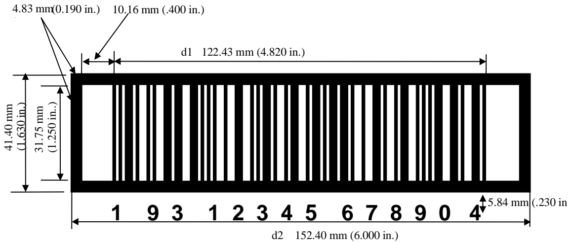
Figure 5-14 ITF-14 symbol size
